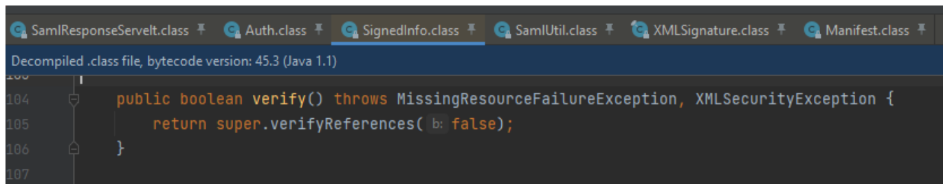
SignedInfo.verify()
