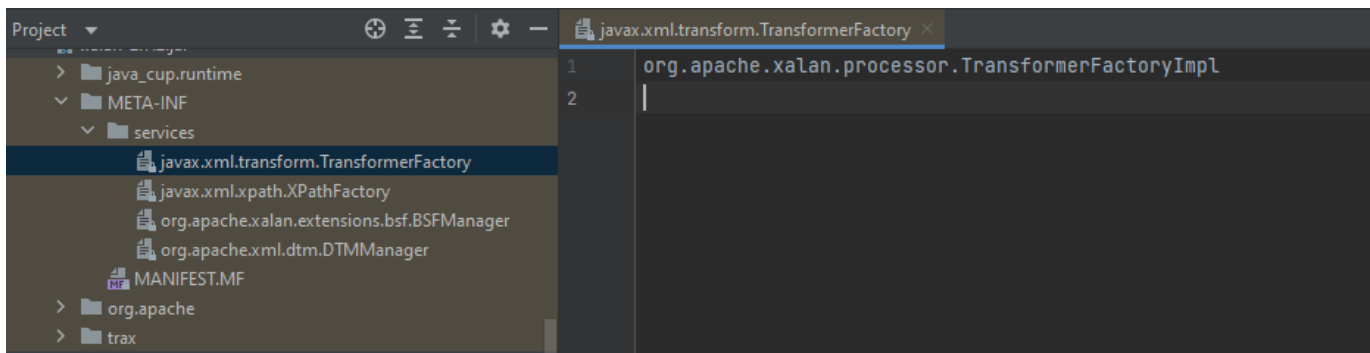
Default TransformerFactory
