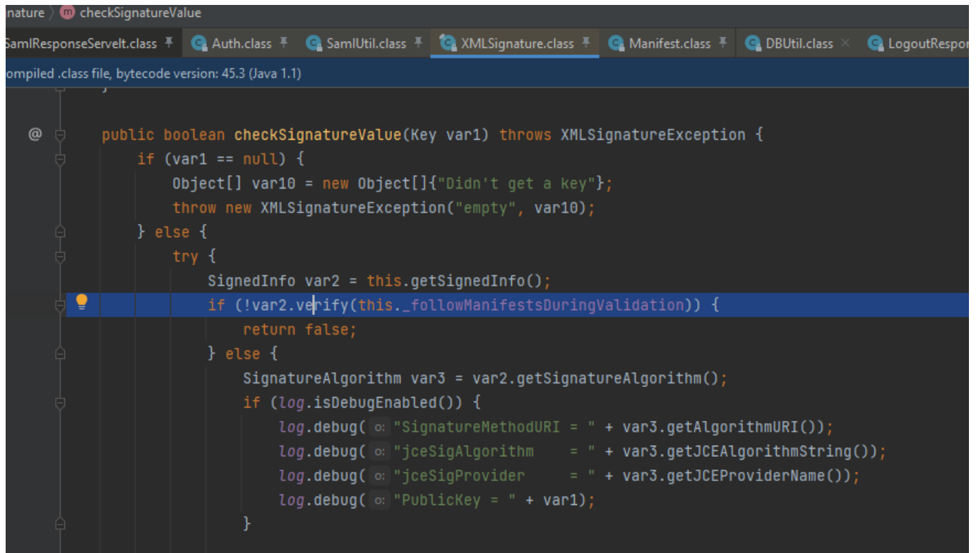
XMLSignature.checkSignatureValue()
