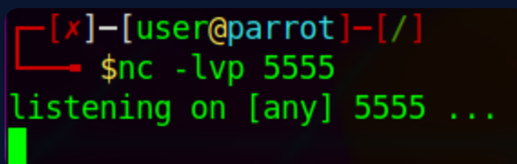
Netcat listening
